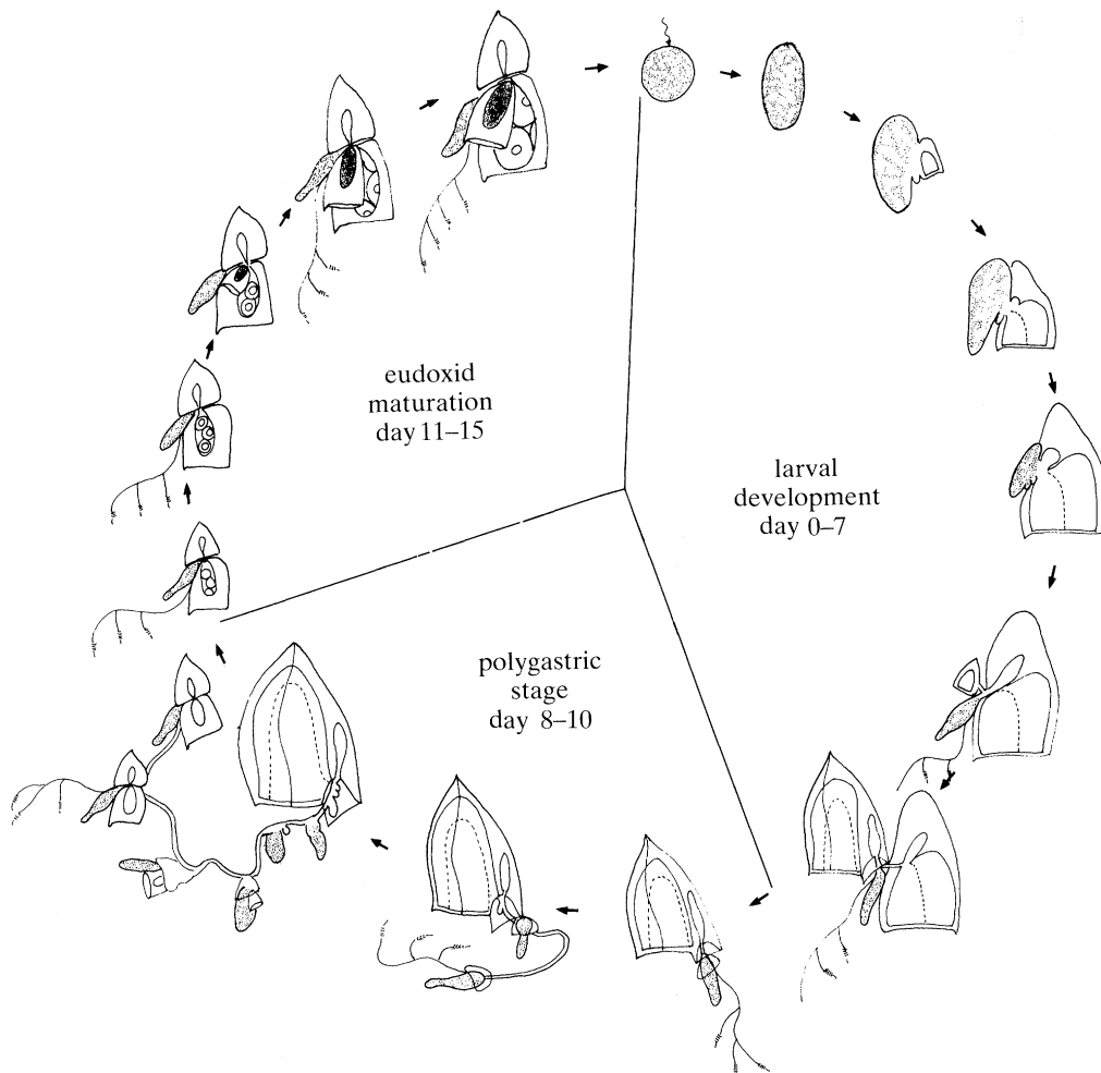
Figure 3. Diagram of complete developmental cycle of Muggiaea kochi with the duration of the larval, polygastric and eudoxid phases at 24 °C.
